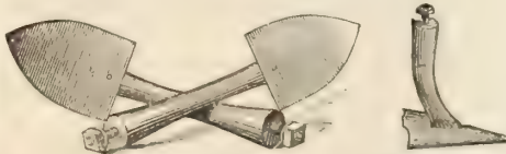
SHOVEL PLOWS.
